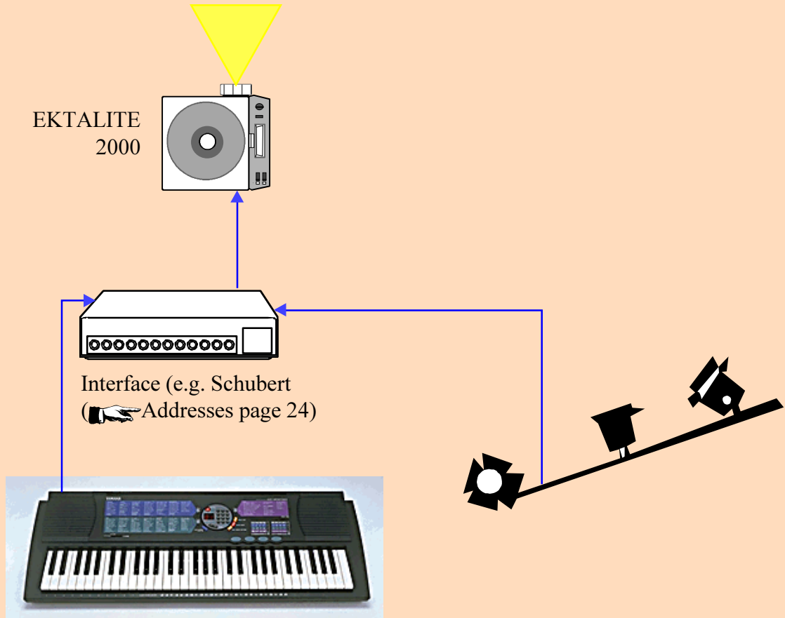
Keyboard with MIDI Interface
